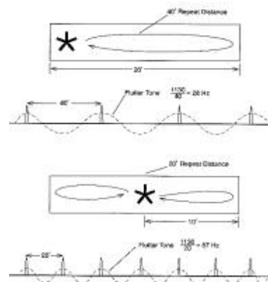
FLUTTER TONE FREQUENCIES
