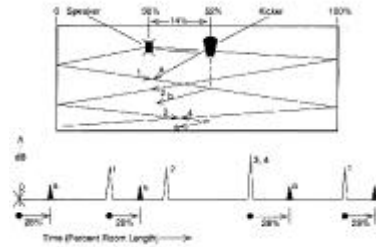
FLUTTER WITH FORWARD KICKER
