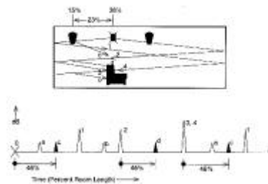
FLUTTER WITH KICKER ADDED
